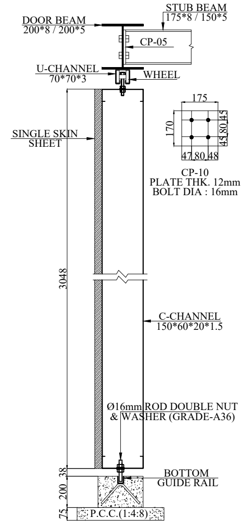
DOUBLE SLIDING DOOR SECTION DETAILS
