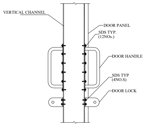
DOOR LOCK AND HANDLE DETAIL
